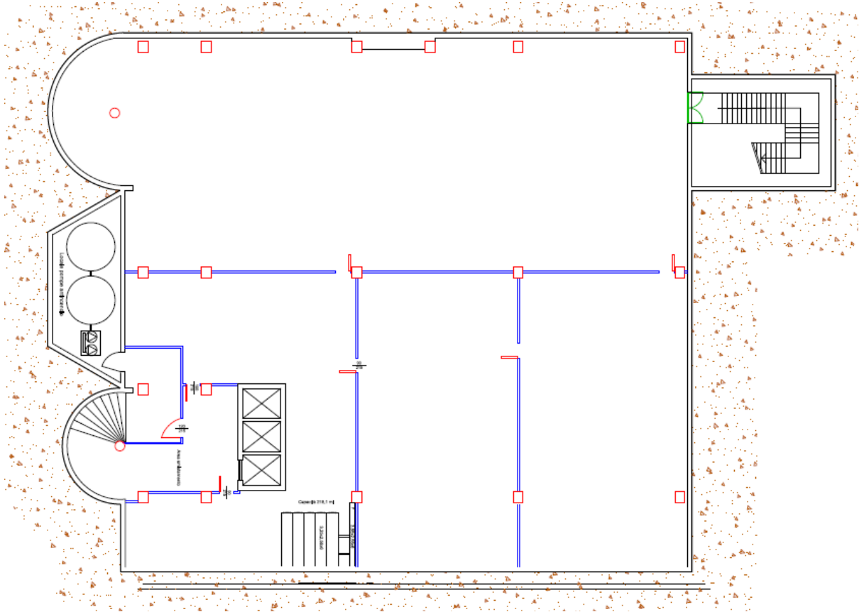
PIANO CANTINATO
